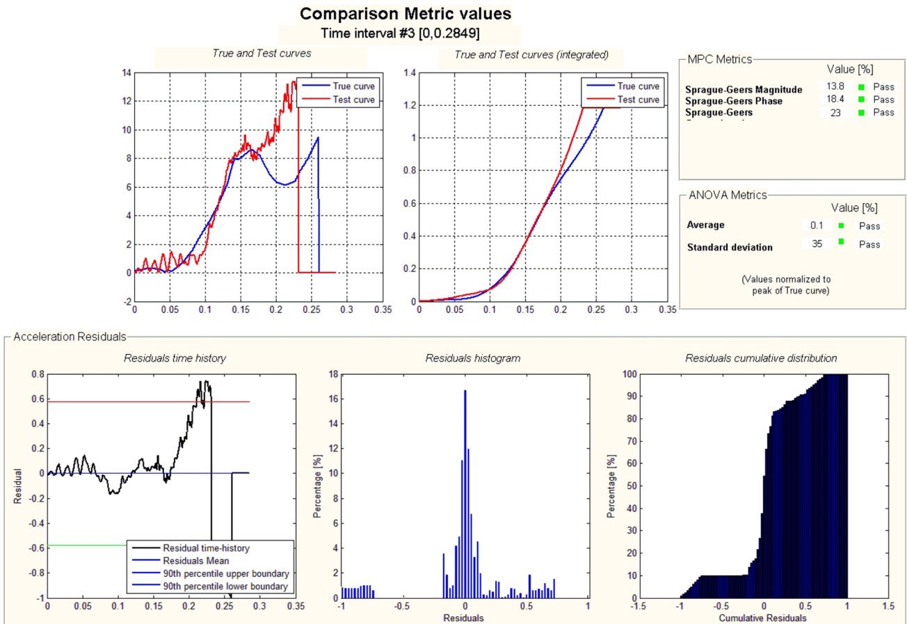
Fig. 12 Comparison of THV curves using RSVVP code: blue—full-scale crash test; red—simulation
