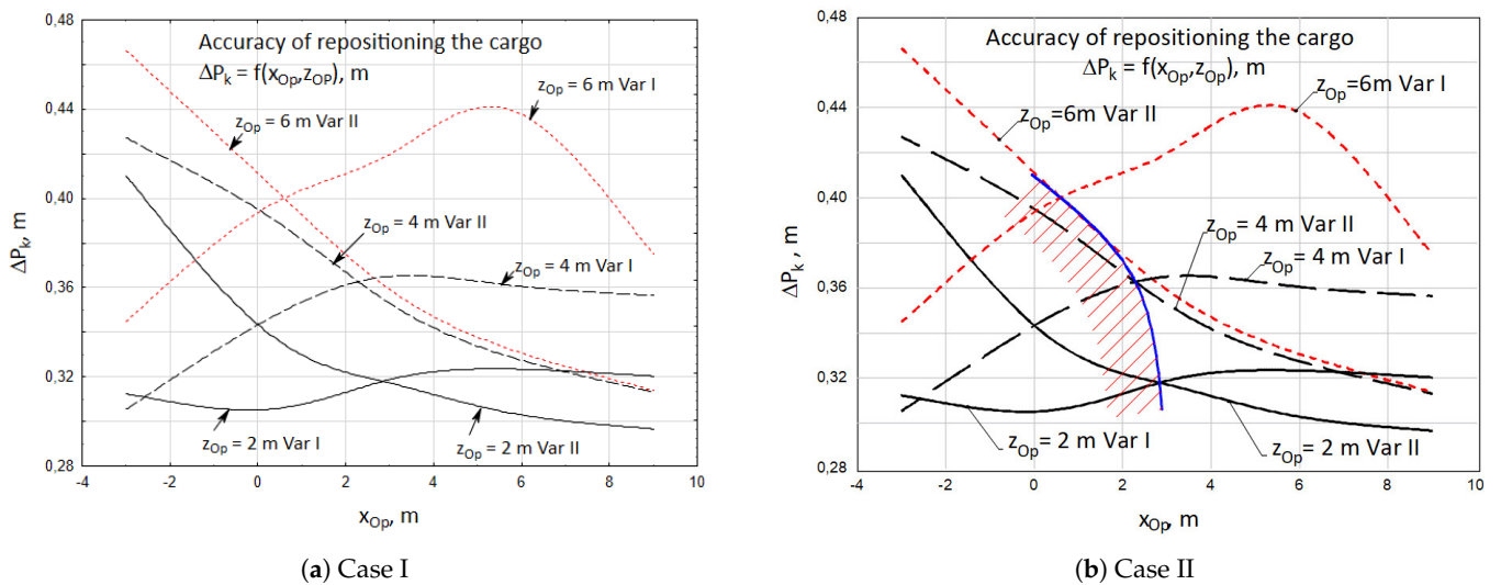
Figure 16. Accuracy of repositioning the cargo \Delta P_k , for two cases of the realized cargo handling task.
