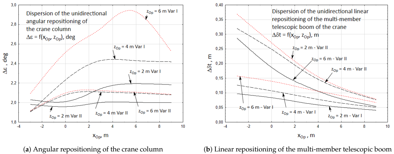
Figure 15. Accuracy of the unidirectional positioning of the cargo.
