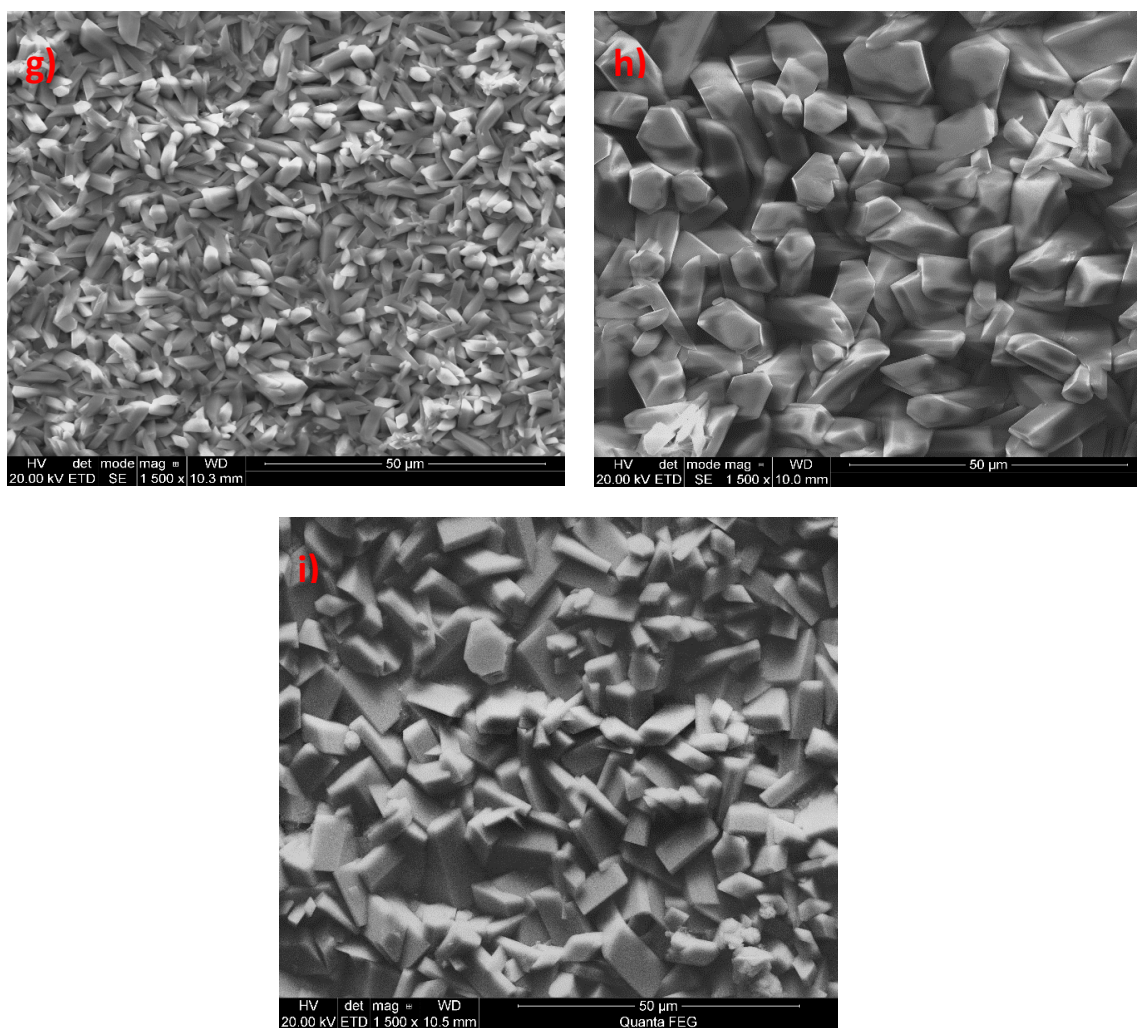
Figure 2. SEM image of the manganese phosphate coating: (a) modified with: \text{Na}_2\text{MoO}_4 , 1500× magnification (b), \text{CaCO}_3 , 1500× magnification (c), \text{Sr}(\text{NO}_3)_2 , 5000× magnification (d), \text{ZnO} , 5000× magnification (e), \text{Cu}(\text{NO}_3)_2 , 10,000× magnification (f), \text{Ba}(\text{NO}_3)_2 , 1500× magnification (g), \text{CdO} , 1500× magnification (h), and \text{Ce}(\text{NO}_3)_2 , 1500× magnification (i).
