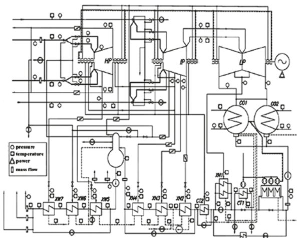
Figure 1. General block diagram including location of the measuring points.
