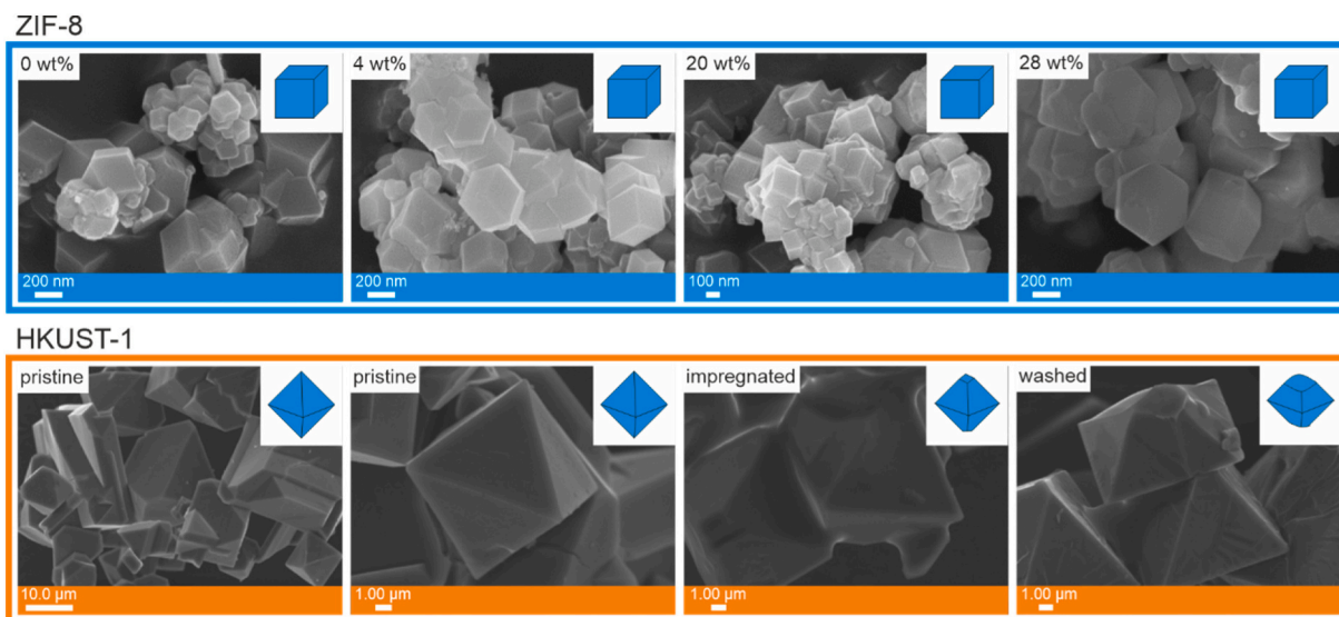
Fig. 30. SEM images of intergrown cubes of ZIF-8 samples impregnated with different amount of [BMIM][BF 4 ] (reproduced from [168]) and distorted octahedrons of HKUST-1 samples treated with [EMIM][Tf 2 N] (reproduced from [157]).
