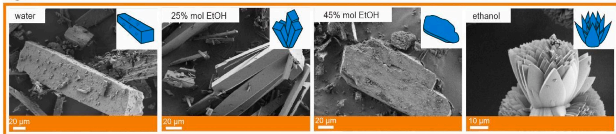
Fig. 15. Dependence of Cu-BTC morphology on the composition of the reaction solution; from left: water – tagliatelle-like structure, water + ethanol – octahedra, ethanol + octanol – sphere, water + DMF – irregular (reproduced from [119 to 121]). Different morphology of Mg/BTC (SEM images and chain model) depending on the amount of ethanol; from left: water – 1D structure, 25%, 45% mol EtOH – 2D structure, ethanol – 3D structure, flower-like structure (reproduced from [124]).
