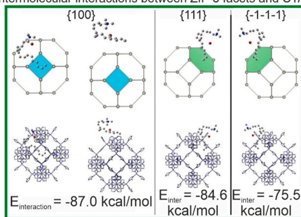
Fig. 22. Different morphologies of MOF-5 (cubes [144] prepared without any modulator and octahedral nanocrystals in a presence of CTAB [145]) and ZIF-8 (rhombic dodecahedrons prepared without any additives, (cubes prepared in the presence of CTAB), (reproduced from [138])); intermolecular interactions between the ZIF-8 facets of and CTAB obtained by semiempirical methods PM6 and PM7 methods included in MOPAC2012 (reproduced from [146]).
