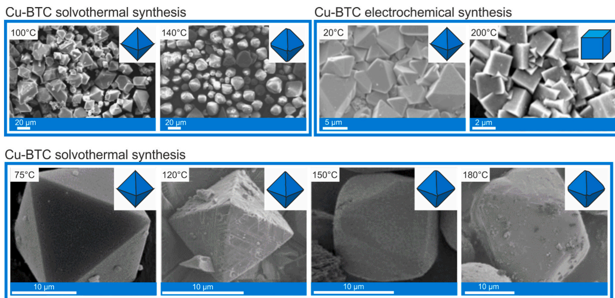
Fig. 10. SEM images of Cu-BTC prepared by solvothermal and electrochemical methods at different temperature conditions. First group of SEM images: left - sharp edges octahedra, right - smooth edges octahedra; second group: left - octahedra, right - cube; third group: left - sharp edges octahedra next ones smooth edges octahedra (reproduced from [82,85,86]).
