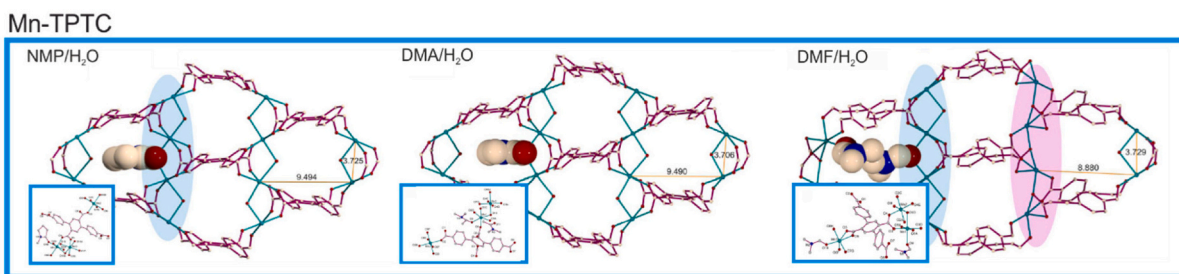
Fig. 18. Models of 1D channels in Mn-TPTC, deposited by H 2 O and NMP/DMA/DMF solvent molecules and the coordination environment of Mn(II) ion MOFs (in boxes, gray C, red O, blue N, cyan Mn (reproduced from [128])).
