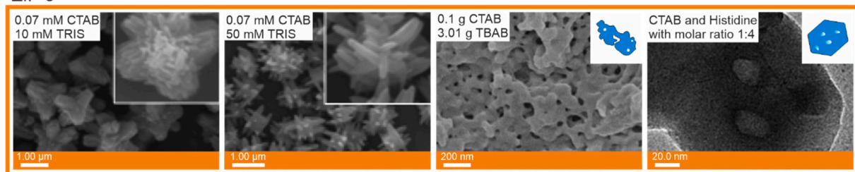
Fig. 24. Morphologies of MOF-5 crystals synthesized with 20-fold diluted synthetic solutions with different concentrations of PVP [150], from left: cubes, truncated cubes, truncated cuboctahedrons, octahedrons; ZIF-8 obtained in the presence of CTAB and various additives (reproduced from [146,152,153]), from left hexapod morphology, sort of burr puzzle, stackable particles, hierarchically structured hexagons.
