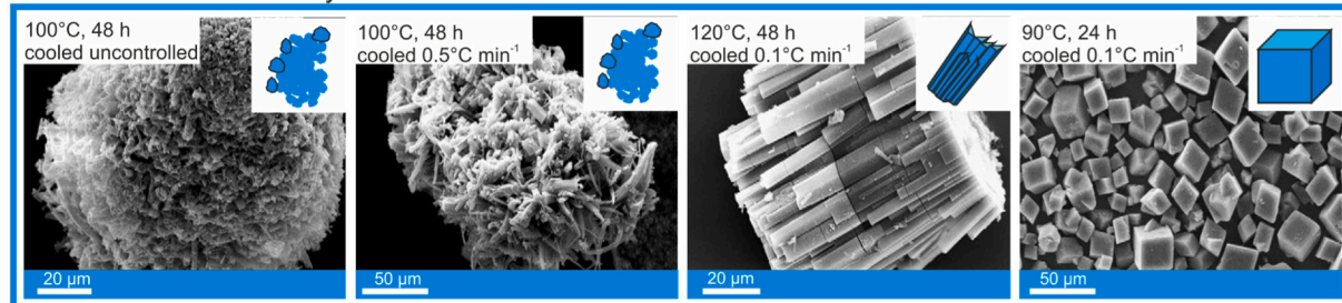
Fig. 11. Effect of heating temperature on morphology of Cu-BDC nanosheets - ultrathin nanosheets, thicker structures of platelets and cube-shaped structures respectively (reproduced from [88]), Ni-MOF - urchin-like structures, neuron-like structures and microwires, respectively (reproduced from [87]), and the combined effect of heating temperature and cooling rate of during formation of MOF-177 ( \text{ZnO}_4(\text{BTB})_2 ) - aggregated microfilaments, aggregated microfilaments and micro-needles and cubes, respectively (reproduced from [92]).
