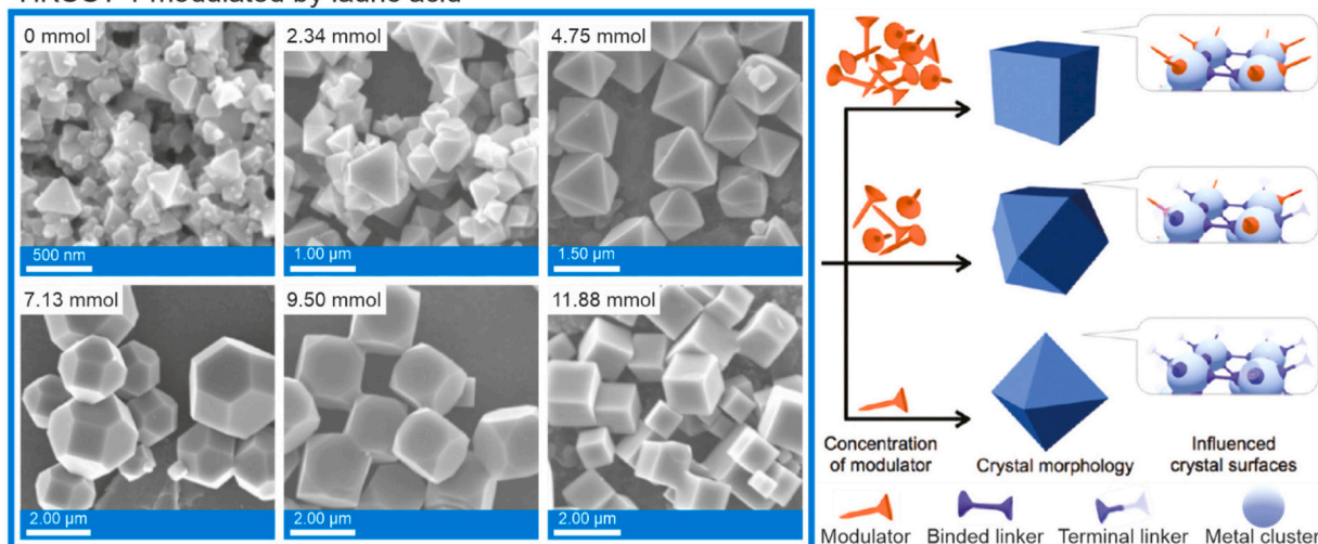
Fig. 23. On the left: morphology transition of [\text{Cu}_3(\text{BTC})_2]_n synthesized in a presence of increasing amount of lauric acid (reproduced from [149]); first row from left: deformed octahedrons, deformed octahedrons, octahedrons; second row: cuboctahedron, truncated cubes, cubes; On the right: schematic illustration of the effect of different modulator (orange symbols) amounts on the coordination process to the MOFs network. The growing concentration of modulator is consequently replacing the terminal linkers (white-blue symbols) and preventing from further growth in specific directions.
