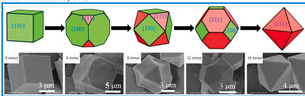
Fig. 21. Schematic and SEM images of the morphology evolution of the IRMOF-3 polyhedral crystals from cubes through truncated cube, cuboctahedron, truncated octahedron to octahedron prepared in the presence of different amounts of CTAB: green facets represent {100}, red facets represent {111} (reproduced from [143]).
