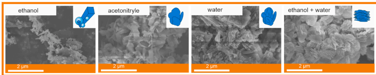
Fig. 16. Shape dependence of Cu-BDC on the solvent used in the synthesis; from left: propionitrile and acetonitrile – 2D nanoplates, 2-propanol and methanol – 3D structure). Shape dependence of Cu-PYDC crystals on solvent composition, PYDC is pyridine-2,5-dicarboxylic acid; ethanol – nanorods, acetonitrile – flakes, water and ethanol + water – irregular, agglomerated particles (reproduced from [88,125]).
