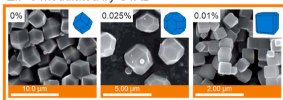
Fig. 22. Different morphologies of MOF-5 (cubes [144] prepared without any modulator and octahedral nanocrystals in a presence of CTAB [145]) and ZIF-8 (rhombic dodecahedrons prepared without any additives, (cubes prepared in the presence of CTAB), (reproduced from [138])); intermolecular interactions between the ZIF-8 facets of and CTAB obtained by semiempirical methods PM6 and PM7 methods included in MOPAC2012 (reproduced from [146]).
