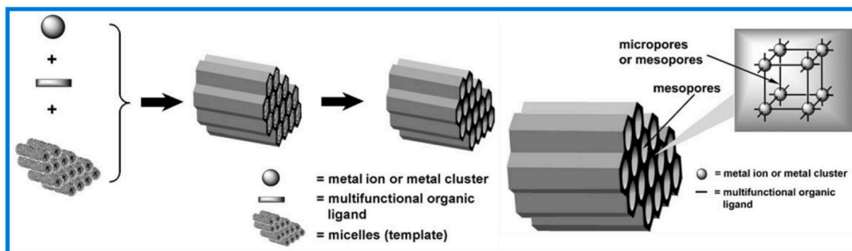
Fig. 26. Formation of mesostructured HKUST-1 by the CTAB templated method (reproduces from [140]).
