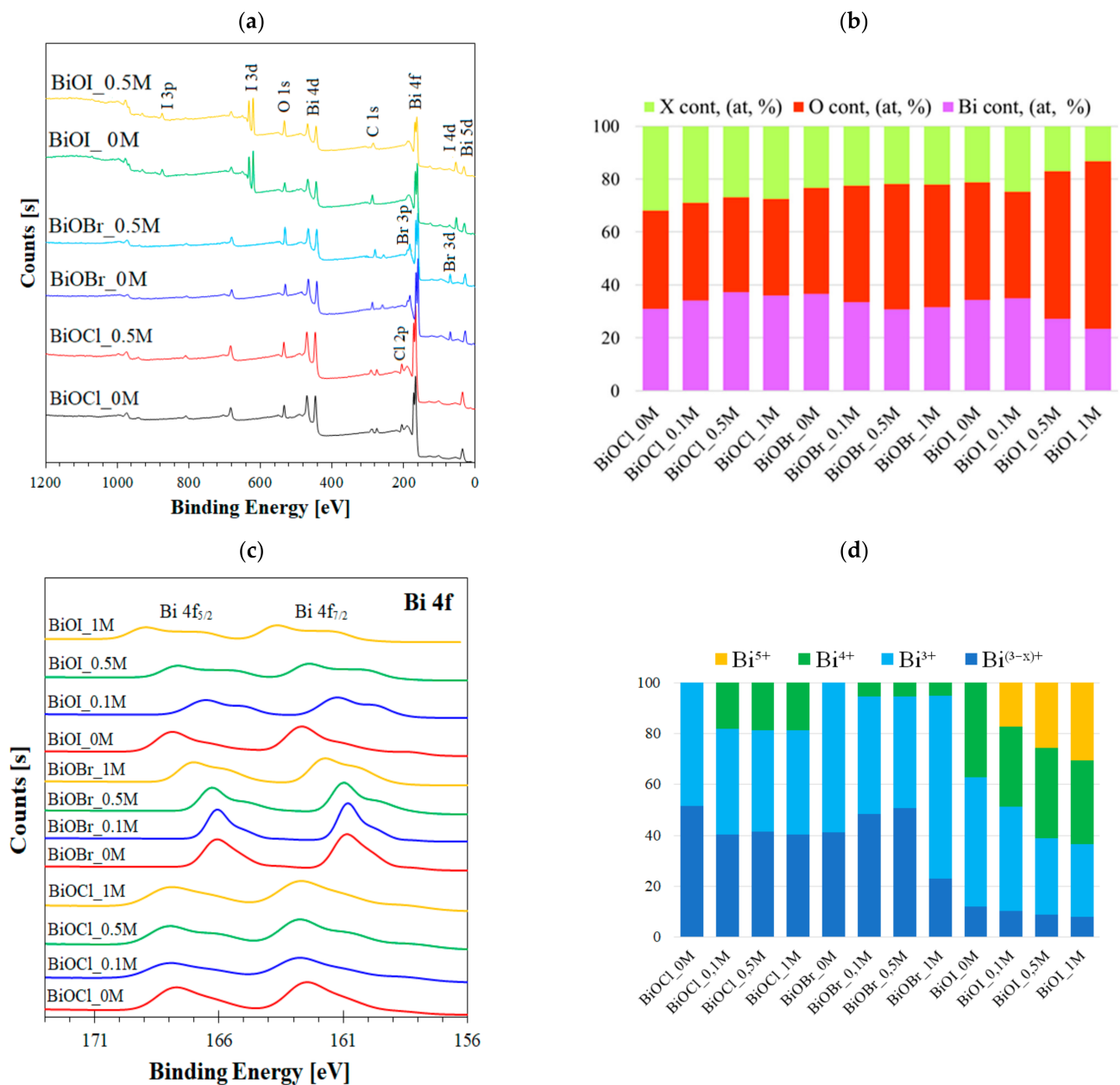
Figure 3. (a) Survey spectra of selected BiOX (X = Cl, Br, I); (b) surface elemental composition of BiOX (X = Cl, Br, I); (c) effect of mannitol on high-resolution spectra of Bi 4f in BiOX (X = Cl, Br, I); and (d) the concentration of mannitol resulting in the bismuth species ratio.
