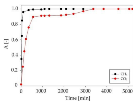
Figure 11. Absorption curves for methane and carbon dioxide in C:DA (1:1).
