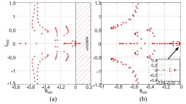
Fig. 3. Spectrum of matrix A of the linearized observer system. The rotor speed is changing from -1.0 to 1.0 p.u., T_L = 0.8 p.u., a) c_\alpha = 5 , c_\psi = 0.5 , \gamma = 0.5 , \gamma_1 = 0 , k_c = 0 . b) c_\alpha = 5 , c_\psi = 0.5 , \gamma = 0.5 , \gamma_1 = 1 , k_c = 0.5 .
