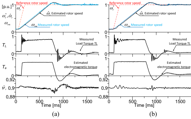
Fig. 10. IM is starting-up to 1.0, nonloaded and the rotor speed value is estimated from (a) adaptive-estimation law (28), (b) nonadaptively (48), the measured load torque T_L waveform is presented.
