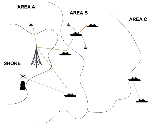
FIGURE 4. Communication areas of the netBaltic system (after [58]).
