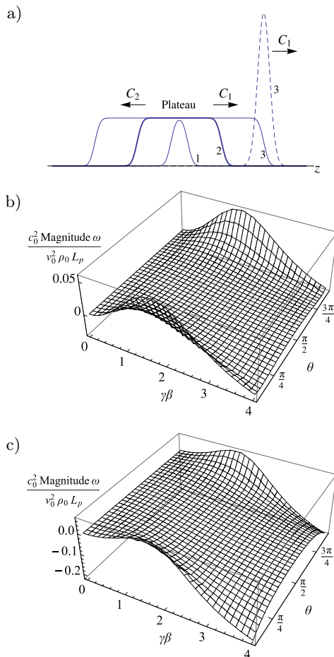
Fig. 3. (a) Drafts of \rho_2 (exaggerated) excited by v_{z,1} = v_0 \exp(-(\omega t - kz)^2) at three consecutive times ordered as 1, 2, 3. An exciting perturbation of density \rho_1 is shown by the dotted line. Below: dimensionless magnitude of the plateau as a function of plasma- \beta and \theta . Cases of L(p) (b) and L(\rho) (c).
