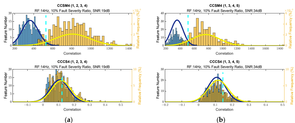
Figure A42. (a) Histograms of diagnostic features for (1,2,3,4) harmonics. (b) Histograms of diagnostic features for (1,3,4,5) harmonics.
