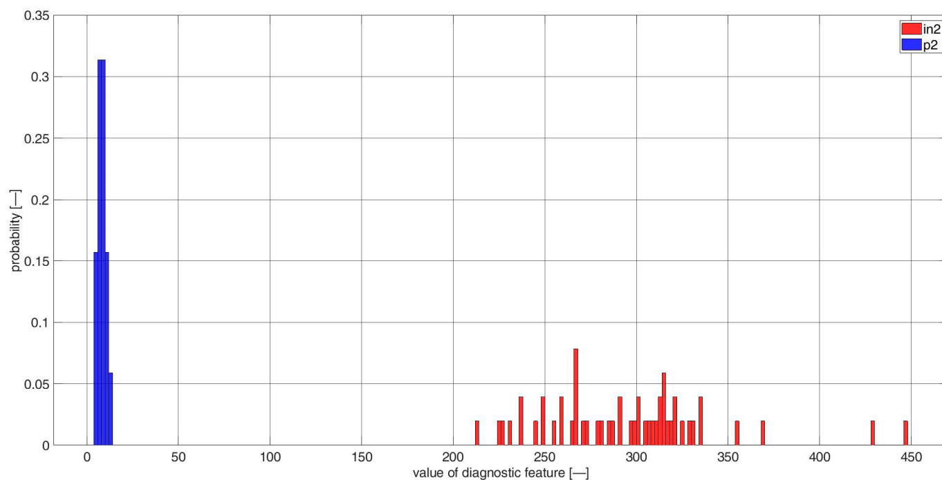
Figure A26. Histogram of diagnostic features based on the CCSM3 (correlation number is 24—Table A1), bearings in2 and p2.
