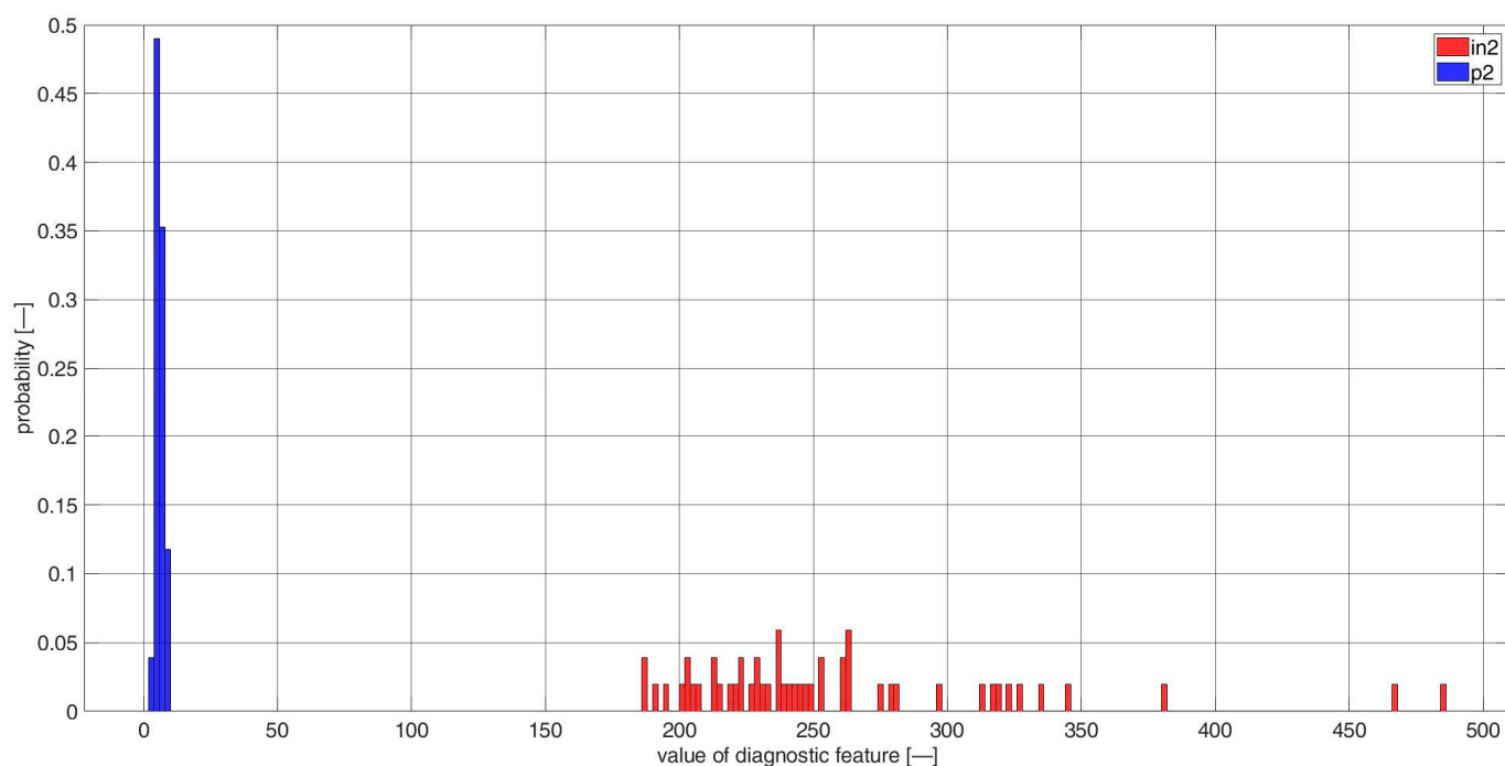
Figure A6. Histogram of diagnostic features based on the CCSM3 (correlation number is 6—Table A1), bearings in2 and p2.
