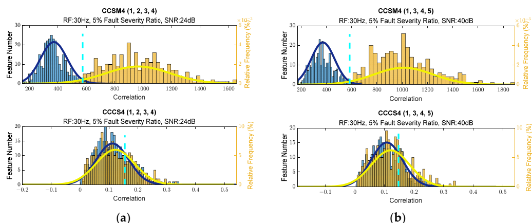
Figure A41. (a) Histograms of diagnostic features for (1,2,3,4) harmonics. (b) Histograms of diagnostic features for (1,3,4,5) harmonics.
