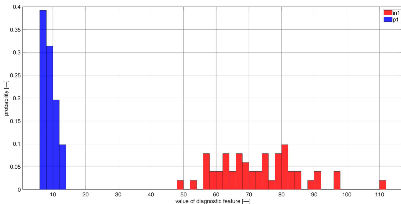
Figure A5. Histogram of diagnostic features based on the CCSM3 (correlation number is 6—Table A1), bearings in1 and p1.
