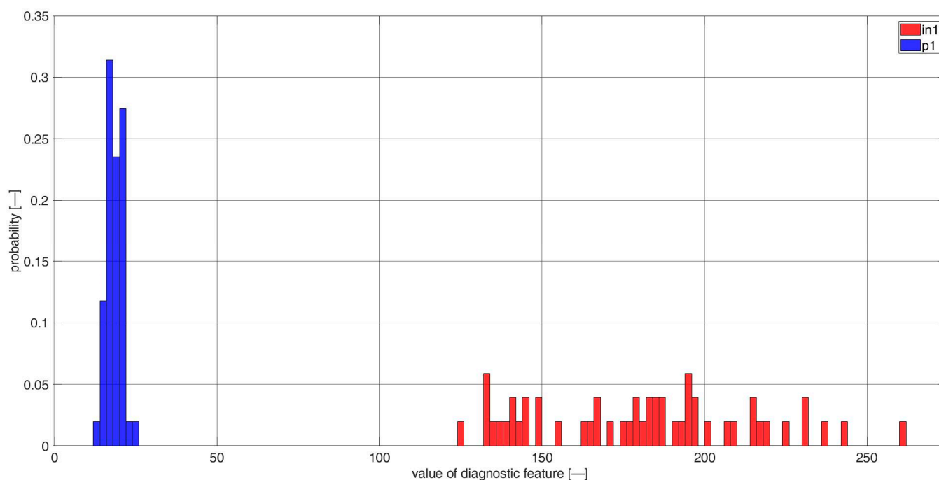
Figure A13. Histogram of diagnostic features based on the CCSM3 (correlation number is 12—Table A1), bearings in1 and p1.
