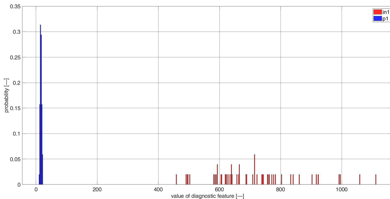
Figure A25. Histogram of diagnostic features based on the CCSM3 (correlation number is 24—Table A1), bearings in1 and p1.
