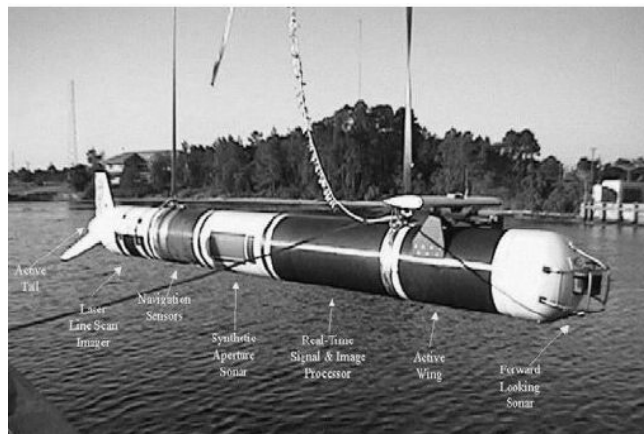
Rys. 14. System MUDSS z gradiometrem SQUID Fig. 14. MUDSS system with SQUID gradiometer
