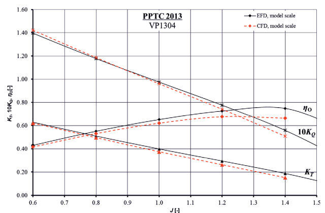
Fig. 3. Comparing experimental data and numerical results for model scale
