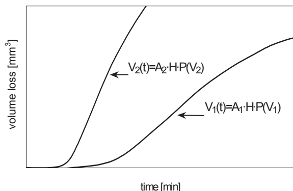
Fig. 6. Influence of eroded area quantity on the volume loss of material for the same intensity of cavitation loading
