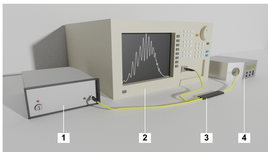
Figure 2. Experimental setup, where: 1—light source, 2—Optical Spectrum Analyzer, 3—Optical fiber coupler, 4—Temperature calibrator.
