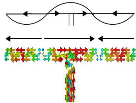
FIGURE 4. Surface current of the dipole driven element at 28 GHz.
