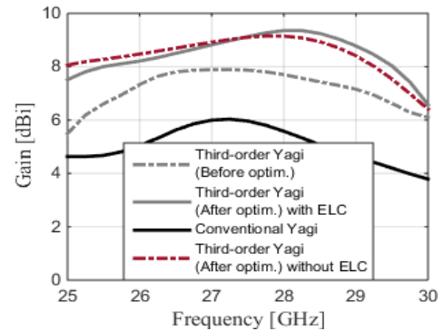
FIGURE 3. Gain plots of the conventional Yagi and third-order Yagi before and after optimization.
