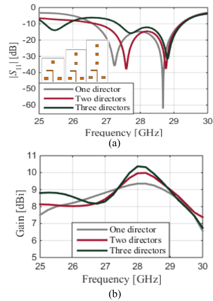
FIGURE 6. The antenna performance with an increasing number of directors: (a) the reflection coefficients and (b) the gain.
