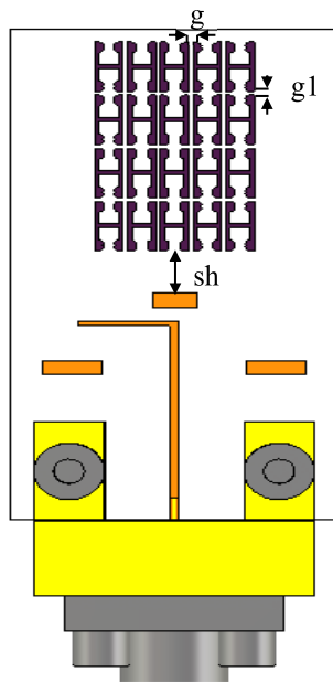
FIGURE 7. The proposed Yagi antenna with a metamaterial array.
