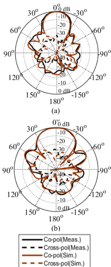
FIGURE 16. Co- and cross-polarization radiation patterns at 28 GHz (a) E-plane and (b) H-plane.
