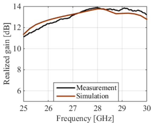
FIGURE 15. Comparison of simulated and measured gains.
