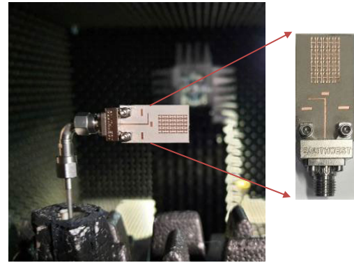
FIGURE 13. Yagi antenna setup in the anechoic chamber, with the inset displaying a close-up of the fabricated prototype.
