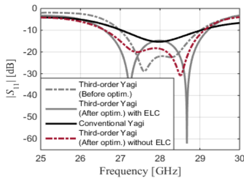
FIGURE 2. Reflection coefficients of the conventional Yagi and third-order Yagi before and after optimization.
