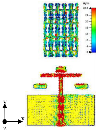
FIGURE 12. Surface current distribution of the metamaterial antenna at 28 GHz.
