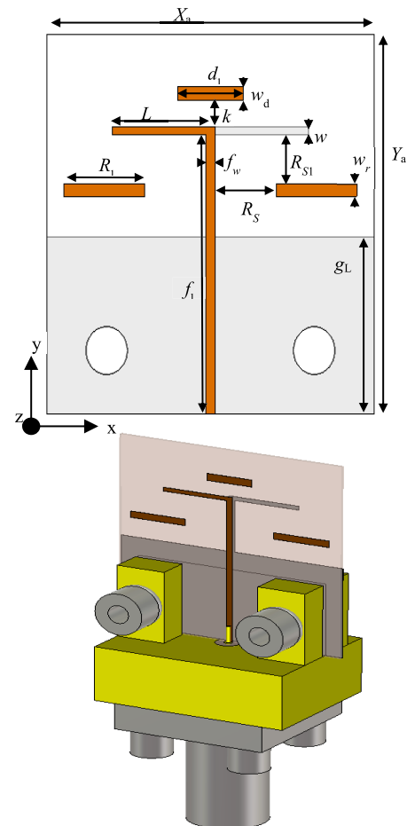
FIGURE 1. The configuration of the Yagi antenna, dimensions; X_a = 15 , Y_a = 17 , L = 4.189 , w = 0.293 , d_1 = 2.058 , w_d = 0.828 , R_L = 2.705 , w_r = 0.828 , R_S = 3.143 , R_{S1} = 1.9 , f_w = 0.388 , f_i = 11.346 , and g_L = 6.522 , k = 0.649 . All dimensions are in mm.
