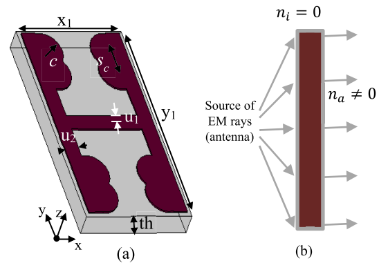
FIGURE 9. (a) Metamaterial configuration. (The dimensions are: x_1 = 1.390 mm, y_1 = 2.820 mm, c = 0.200 mm, sc = 0.204 mm, u_1 = 0.103 mm, u_2 = 0.203 mm, th = 0.254 mm), and (b) Gain enhancement mechanism.
