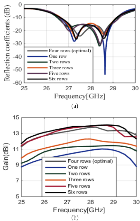
FIGURE 11. Performance of the metamaterial antenna with varying numbers of array rows: (a) reflection coefficient and (b) gain.
