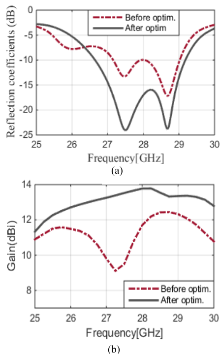
FIGURE 8. Metamaterial antenna performance before and after optimization: (a) Reflection coefficient, and (b) gain.
