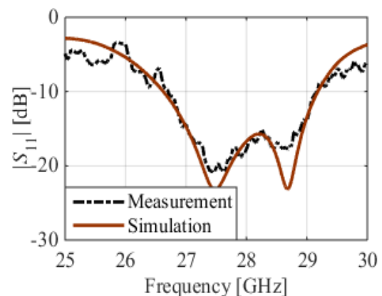
FIGURE 14. Comparison of simulated and measured reflection coefficients.
