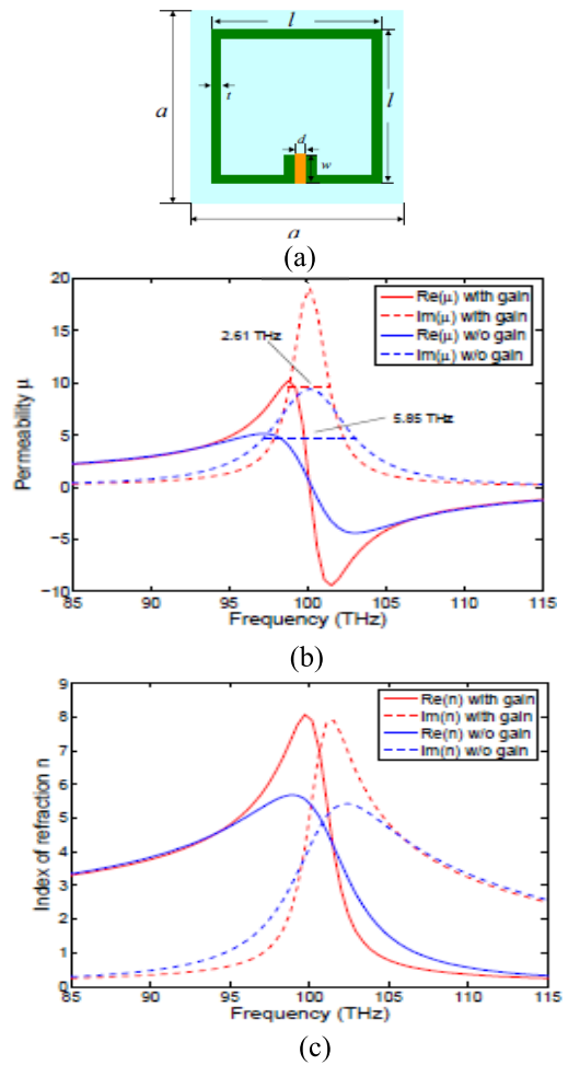
FIGURE 21. SRR incorporated gain material for loss compensation proposed in [128]: (a) schematic view of the SRR with gain embedded in the gap (orange), (b) the retrieved \mu with and without the gain material, and (c) the retrieved refractive index.
