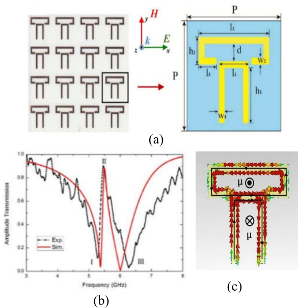
FIGURE 6. EIT-like metamaterial reported in [67]: (a) the array and single unit cell of SRRs, (b) the simulated and measured transmission coefficients, and (c) the surface current distribution at 5.5 GHz.
