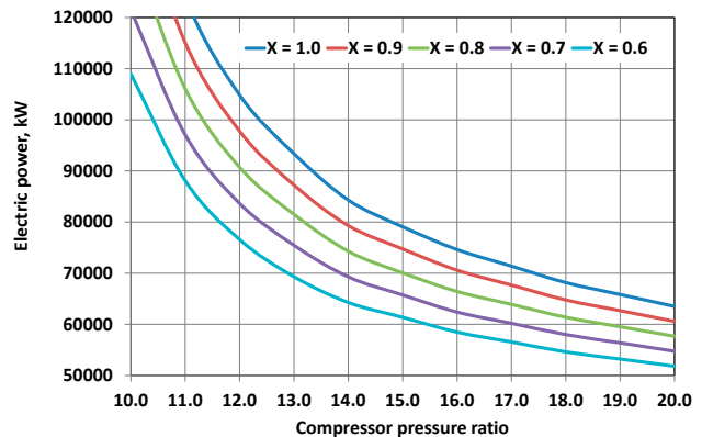
Fig. 7. Dependences of the electric power of the CGSTU on the SIGT compressor pressure ratio and the parameter of the partial steam supply.
