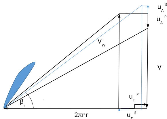
Figure 3. Velocity components on the propeller blade element.
