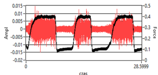
Fig. 7. EMG signal (red) and force (black) in time
