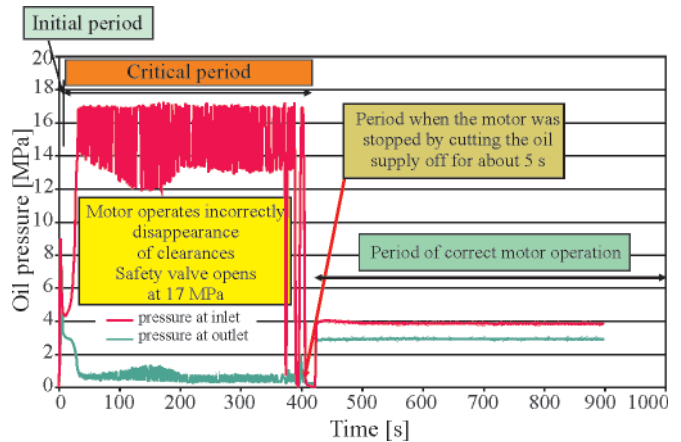
Fig. 16. Oil pressures at motor inlet and outlet: cold chamber temperature t_{ot} = -15 \text{ }^\circ\text{C} , oil temperature t_{oi} = 53 \text{ }^\circ\text{C} , the oil flow rate Q = 100 \text{ [l/min]}
