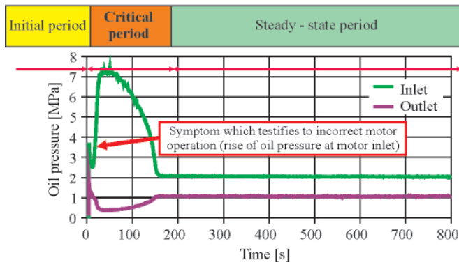
Fig. 15. Oil pressures at motor inlet and outlet: cold chamber temperature t_{ot} = -20 \text{ }^\circ\text{C} , oil temperature t_{oi} = 50 \text{ }^\circ\text{C} , oil flow rate Q = 100 \text{ [l/min]}
