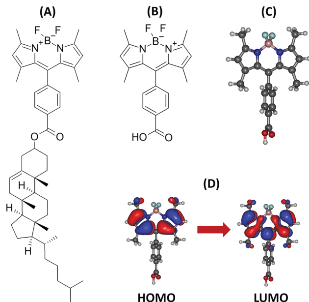
Fig. 1 Structure of the BODIPY-Ar-Chol dye (A), investigated BODIPY compound (B), optimized structure (C), and orbitals involved in the first singlet excited state (D).
