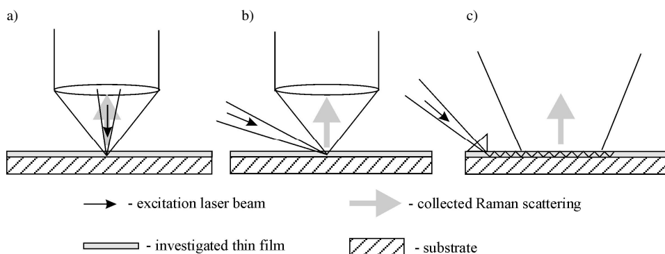
Fig. 2. Optical setups for Raman investigations of thin solid films: a) backscattering configuration, b) glancing-incidence configuration, c) waveguide configuration
