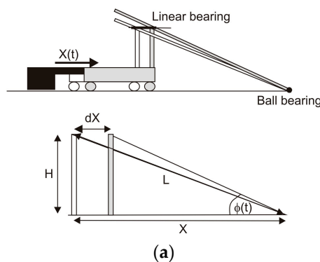
Figure 11. Modified shaking table: (a) scheme (top image) and trigonometric dependence for Equation (9) (bottom image: H = 0.5 \text{ m} , L = 3.7 \text{ m} ); (b) general view of shaking table with mounted FOSREMs and HZ1-100-100.
