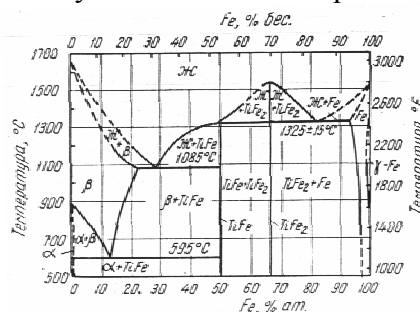
Fig. 1. The equilibrium iron - titanium diagram [5]
