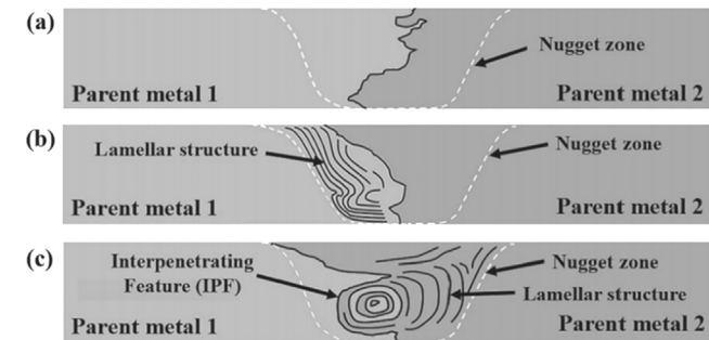
Fig. 24. Schematic illustration of the three characteristic joint macrostructures observed in the dissimilar Al-Mg joints: (a) Type I, distinct boundary, (b) Type II, lamellar structure with distinct boundary, and (c) Type III, complex intercalated lamellar structure [60].
