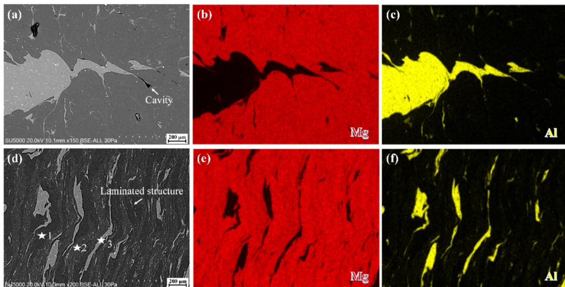
Fig. 49. SEM images and EDS mapping of the microstructure in (a–c) FSW and (d–f) SFSW weld fabricated at 800 rpm [116].
