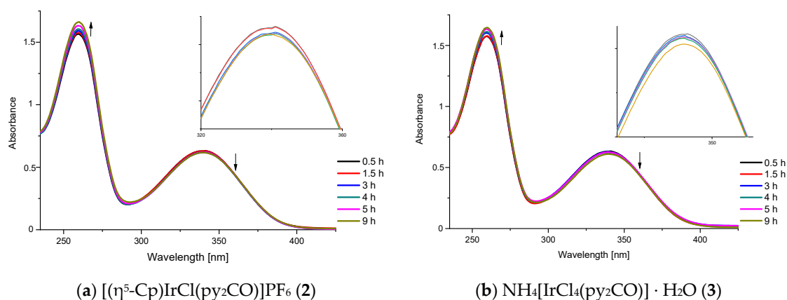
Figure 12. UV-Vis spectra for the catalytic oxidation of NADH ( 100 \mu\text{M} ) to \text{NAD}^+ in the presence of complexes ( 1 \mu\text{M} ) over a 9 h period in 50% MeOH/50% \text{H}_2\text{O} (V:V) (inset: wavelength absorbance changes from 315–360 nm).
