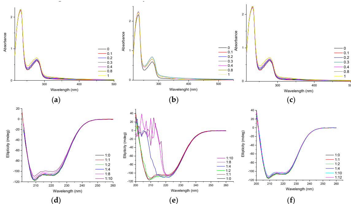
Figure 13. Changes in UV-Vis absorption spectra of HSA ( 2 \times 10^{-5} \text{ M} ) in Tris-HCl/NaCl buffer upon addition of 1 (a), 2 (b) and 3 (c) in different molar ratio and CD spectra of HSA incubated with 1 (d), 2 (e) and 3 (f) in different molar ratio.
