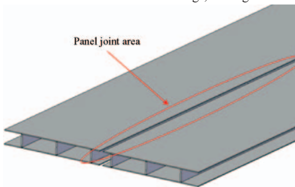
Fig. 2. Positions of I-core panels in longitudinal arrangement.
