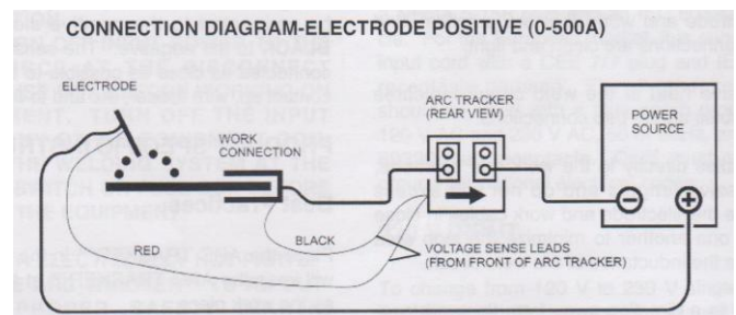
Fig. 1 Connection diagram of Arc Tracker in the experimental set up.[15]
