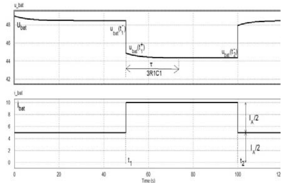
Fig.2. Battery voltage u_{bat} waveform change due to impulsive current i_{bat}
