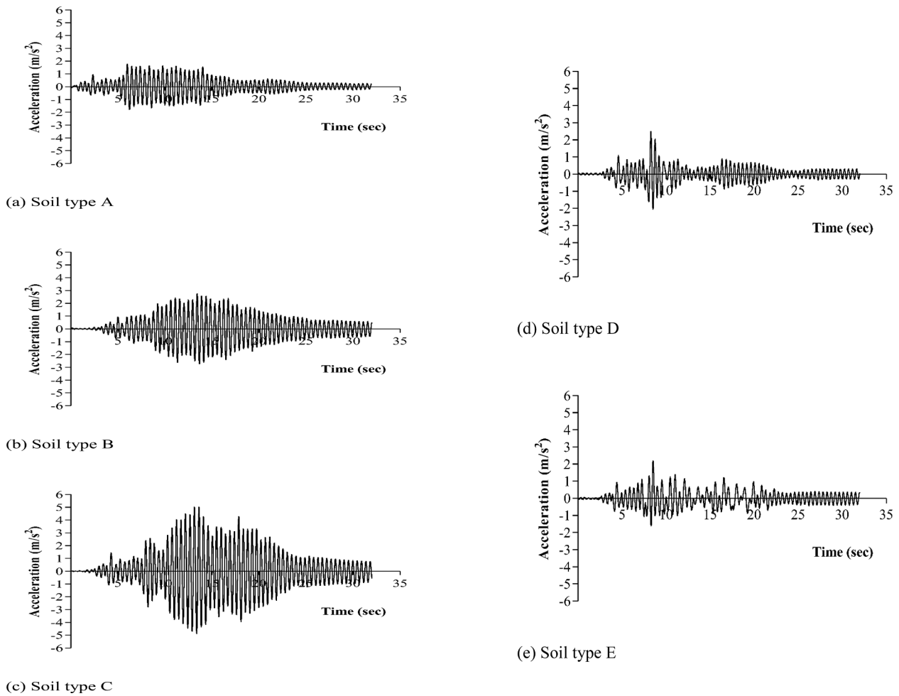
Fig. 8. Acceleration time history of Model 2 under different soil types exposed to the Imperial valley earthquake for the no pounding case.
