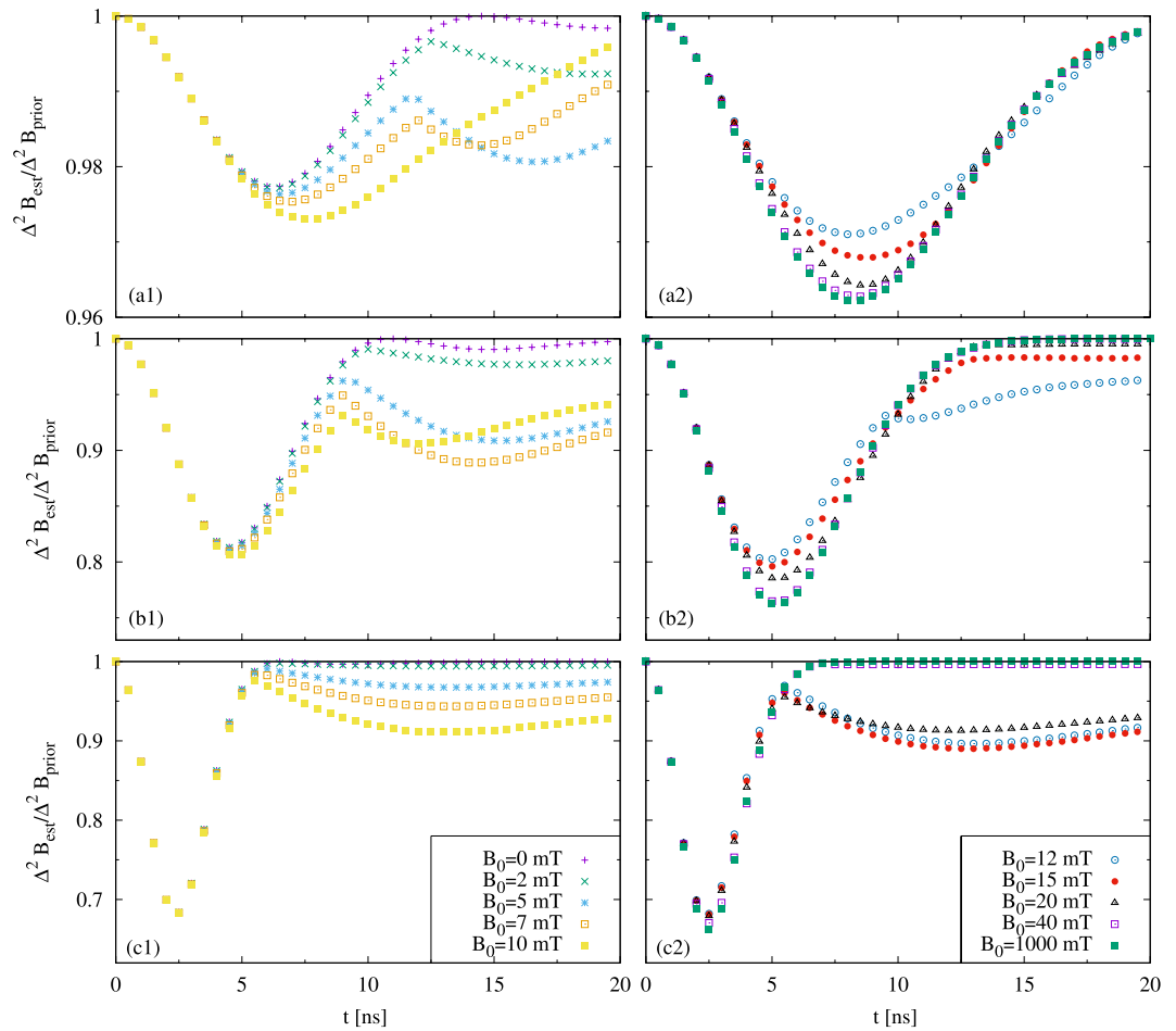
Figure 1. Estimation of B for a single qubit. We plot \Delta^2 B_{est}/\Delta^2 B_{prior} optimized over states, against time, for several values of the mean B_0 and variance \Delta B_{prior} = 1 mT ( a1,a2 ), \Delta B_{prior} = 4 mT ( b1,b2 ), \Delta B_{prior} = 10 mT ( c1,c2 ). For small B_0 there are two time regimes, the phase one to the left and the population one to the right.
