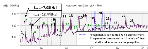
Fig. 4. The ship noise spectrum at the distance marked "0" in Fig. 3.
