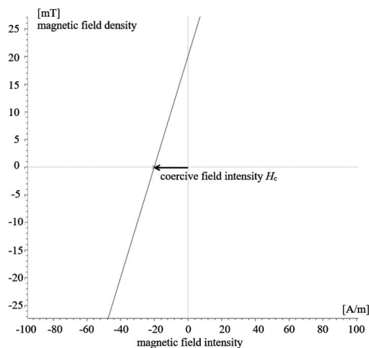
Fig. 6. Offset of the initial magnetization curve.
