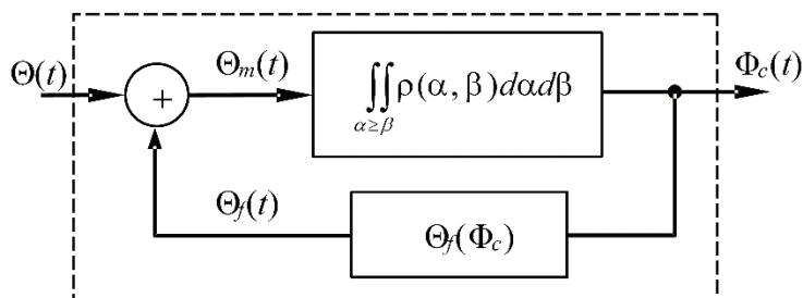
Fig. 4. Block diagram of the feedback hysteresis model
