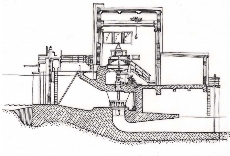
Figure 1. Ptusza hydropower plant, cross section (drawing made on the basis of documentation of WUOZ in Piła).
