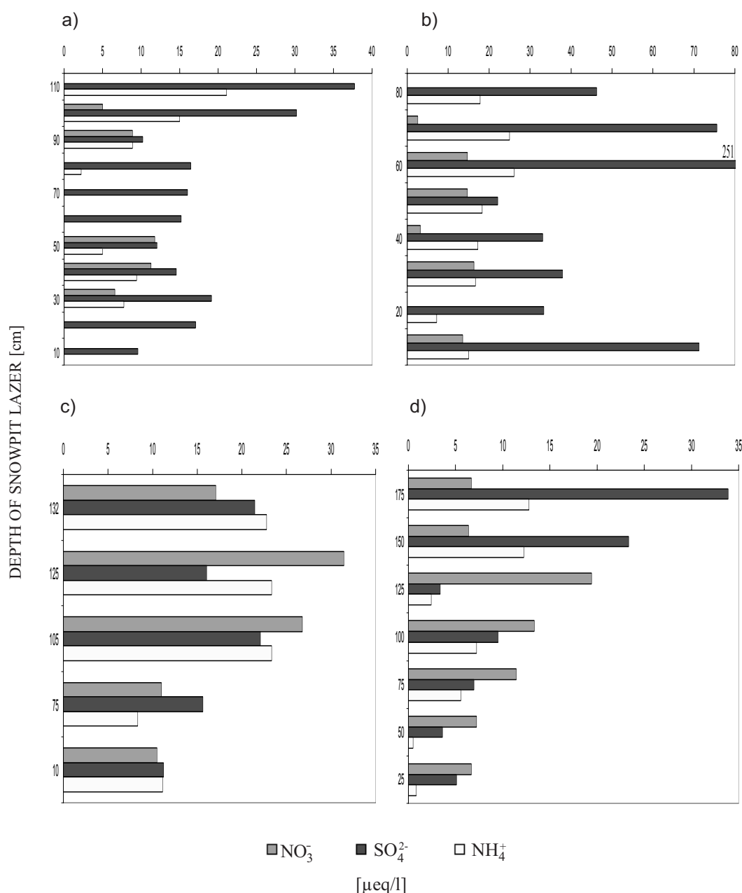
Fig. 9. Mean concentrations of nitrate, sulphate, and ammonium ions in samples of snow collected at a) Śnieżnik, b) Orle, c) Szenia in January 2008 (author's own results), and d) the Alps (April 1994) [32].
