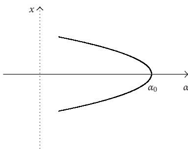
Figure 3.3. Subcritical bifurcation.
