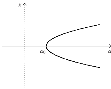
Figure 3.2. Postcritical bifurcation.
