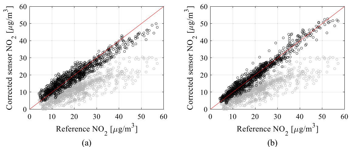
Figure 26. Scatter plots for the testing data (uncorrected—gray, corrected—black): (a) setup B.4, (b) setup D.3.
