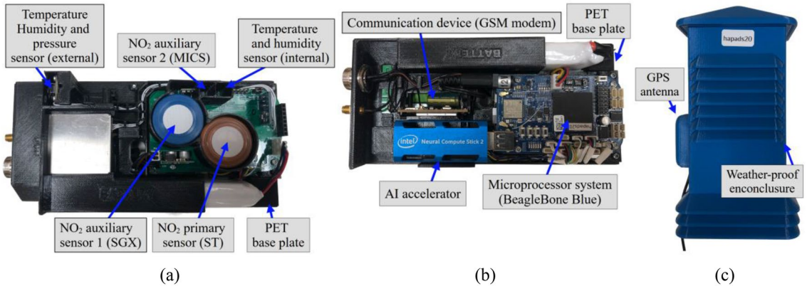
Figure 2. Autonomous monitoring platform designed at Gdansk University of Technology, Poland: (a) internals (top view), (b) internals (bottom view), (c) systems mounted in weather-proof enclosure.
