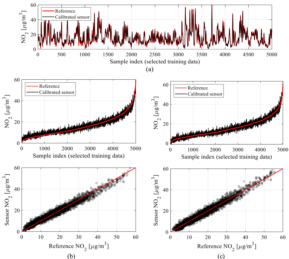
Figure 18. Global response correction: (a) a subset of selected training data; (b) the same data arranged based on increasing \text{NO}_2 reference readings (top) accompanied by the corresponding scatter plot (bottom). Despite the apparent alignment showcased in Fig. 18a, there is an observable systematic offset dependent on the level; (c) the same data after the application of global data scaling, showcasing a notable decrease in the systematic offset and an enhancement in the symmetry of the scatter plot. In this instance, global correction results in an improved correlation coefficient, rising from 0.93 to 0.95, and a reduction in RMSE from 2.1 to 1.8 \mu\text{g}/\text{m}^3 .
