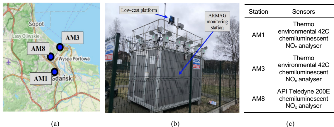
Figure 4. Reference monitoring stations of the ARMAG foundation used to acquire reference data: (a) station locations in the city of Gdańsk, (b) photograph of the selected station with the proposed low-cost platform mounted in the vicinity, (c) NO x sensors installed on the stations.
