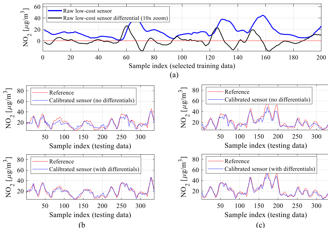
Figure 14. Differentials used as additional ANN surrogate inputs to enhance calibration dependability: (a) selected training data sequence (NO 2 readings from the low-cost sensor) and its corresponding differentials (15); (b) the effects of incorporating differentials shown for a selected sequence of testing data; (c) the effects of differentials shown for another testing data sequence. Note that including differentials (here, of all environmental variables and the primary NO 2 readings from the low-cost sensor) noticeably improves data alignment.
