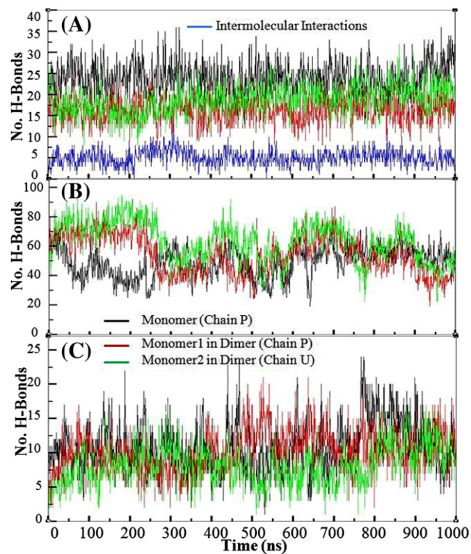
Fig. 3. Hydrogen bond interaction analysis for EmrE monomer (in black color) and dimer systems (red color for monomer1—Chain P) and green color for monomer2—Chain U). Comparison of the number of H-bond contact formed between (A) protein–protein (intramolecular and intermolecular) (B) protein and water molecules, and (C) protein with lipid headgroups. The cutoffs used to define H-bonds are 3.5 Å for the donor–acceptor distance and intermolecular angle values are in range 160°–180° between donor–H–acceptor.
