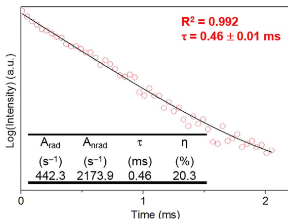
Fig. 8. Luminescence decay curve for calix-TA-Eu ( \lambda_{\text{ex}}=322 nm, \lambda_{\text{em}}=615 nm) and luminescence parameters (inset table).
