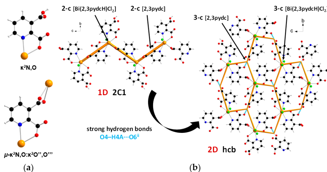
Figure 5. (a) Coordination modes of carboxylate ligands in complex 2; (b) a fragment of the 1D crystal structure merged with 2C1 underlying net in valence-bonded MOFs standard representation and a fragment of the 2D crystal structure merged with hcb underlying the net in H-bonded MOFs standard representation for coordination polymer 2 (Bi—orange, O—red, N—blue, Cl—green, C—black, H—white).
