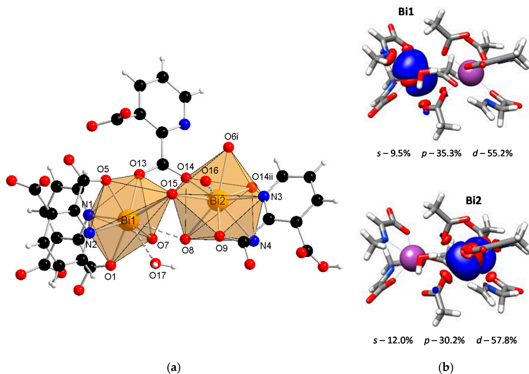
Figure 1. (a) The molecular structure with an atom numbering scheme of complex 1 (Symmetry codes: (i) -x, 1-y, 1-z ; (ii) 1-x, 1-y, 1-z ) (Bi—orange, O—red, N—blue, C—black, H—white); (b) graphical representation of selected molecular orbital localized on Bi atom in complex 1 (DFT calculations).
