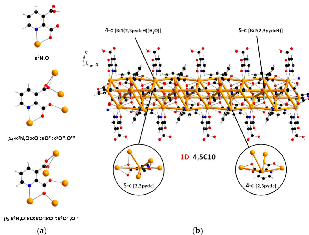
Figure 3. (a) Coordination modes of carboxylate ligands in complex 1; (b) a fragment of the 1D crystal structure merged with 4,5\text{C}10 underlying net in valence-bonded MOFs standard representation for coordination polymer 1 (Bi—orange, O—red, N—blue, C—black, H—white).
