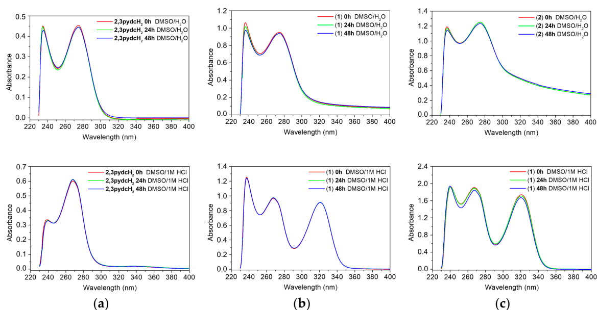
Figure 10. Time-dependent (0 h, 24 h and 48 h) stability studies on: (a) 2,3pydcH 2 , (b) complex 1 , (c) complex 2 in DMSO/H 2 O 1:50 ( v/v ) (top) and DMSO/1M HCl 1:50 ( v/v ) (bottom) solutions monitored by UV-Vis absorption spectra.
