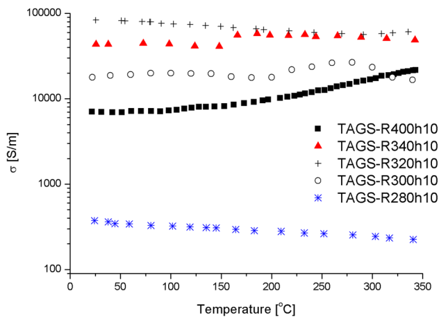
Fig. 4. Temperature dependence of electrical conductivity ( \sigma ) for TAGS85 reduced at various temperatures from 280°C to 400°C for 10 h.
