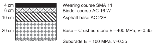
Figure 7. Pavement structure assumed for M-EPDG analysis.
