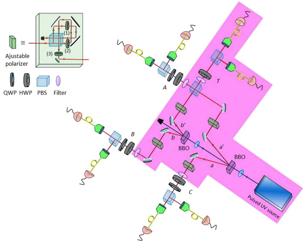
Fig. 6. Experimental setup for the generation of three-qubit polarization bound entangled state. The colored area represents the state preparation. See Methods for more details. QWP, quarter-wave plate; HWP, half-wave plate; PBS, polarizing beam splitter; BBO, \beta -barium borate; UV, ultraviolet.
