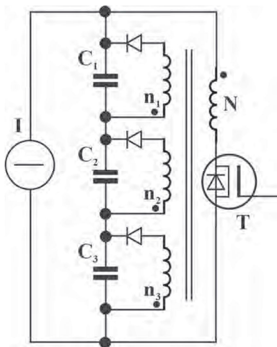
Fig. 6. Equalisation by means of a flyback converter with sectional secondary winding [3].
