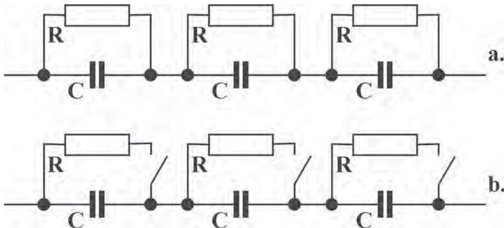
Fig. 3. Standard (a) and improved (b) methods of SC voltage equalisation [1].
