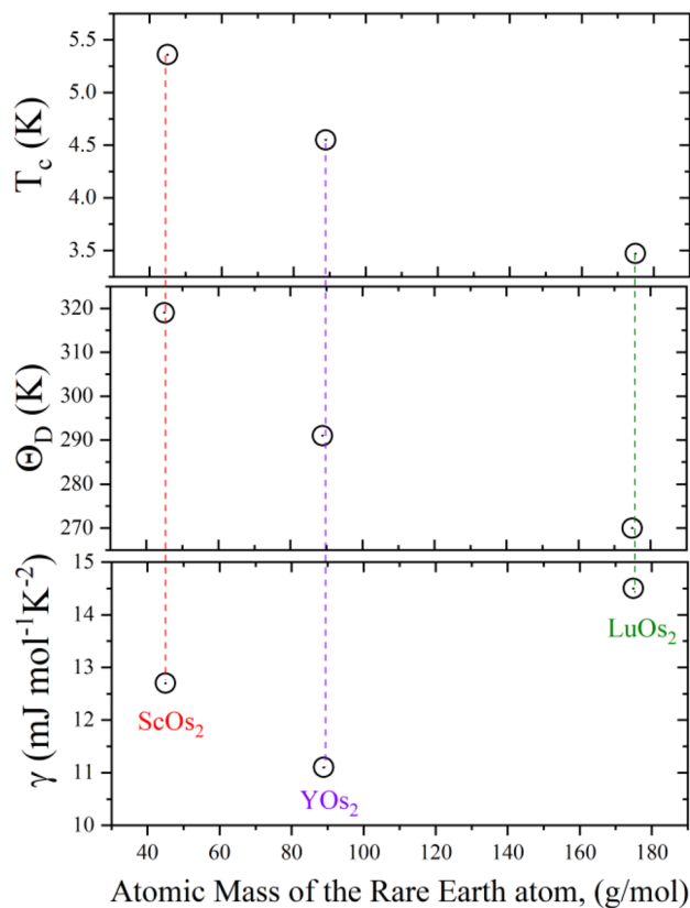
Figure 5. The critical temperature, the Debye temperature, and the Sommerfeld coefficient versus atomic mass of the rare earth atom in ROs_2 compounds ( R = \text{Sc, Y and Lu} ).
