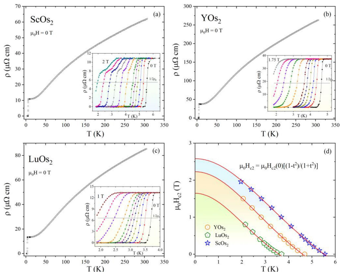
Figure 6. The electrical resistivity versus temperature measured in zero applied magnetic field for \text{ScOs}_2 (a), \text{YOs}_2 (b), and \text{LuOs}_2 (c). Insets show the superconducting transition under various magnetic fields. (d) The temperature dependence of the upper critical field of all compounds, determined from electrical resistivity measurements.
