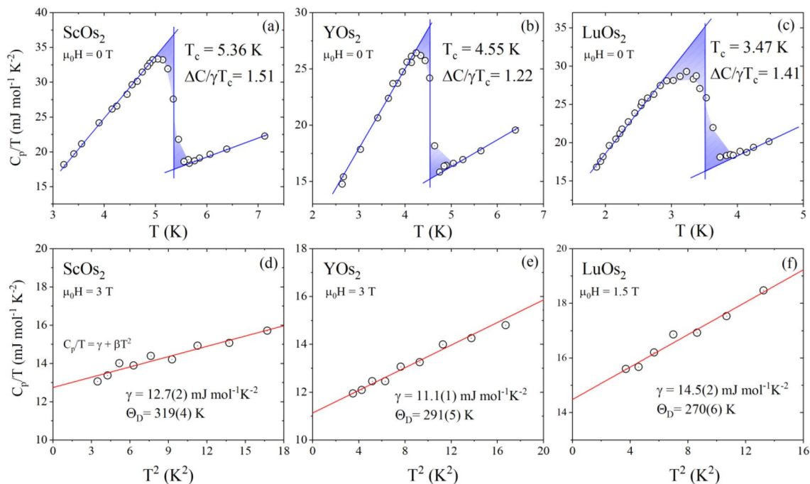
Figure 4. Temperature dependence of the zero-field specific heat in the vicinity of the superconducting phase transition for ScOs 2 (a), YOs 2 (b), and LuOs 2 (c). C_p/T vs T^2 measured in a magnetic field: ScOs 2 (d), YOs 2 (e), and LuOs 2 (f).
