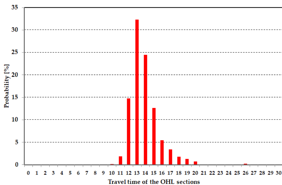
Figure 10. Histogram of the total travel time on OHL sections (TBUS-1 variant).
