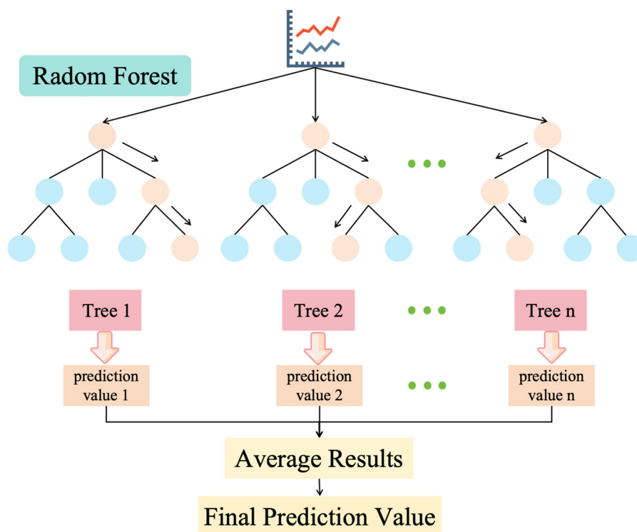
Figure 3: A diagrammatic representation of the RF method [73].
