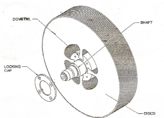
Fig. 1. Rotor of a multidisc Tesla bladeless turbine [3]
