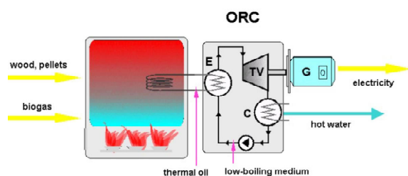
Fig. 2. A cogeneration unit with an ORC system:
